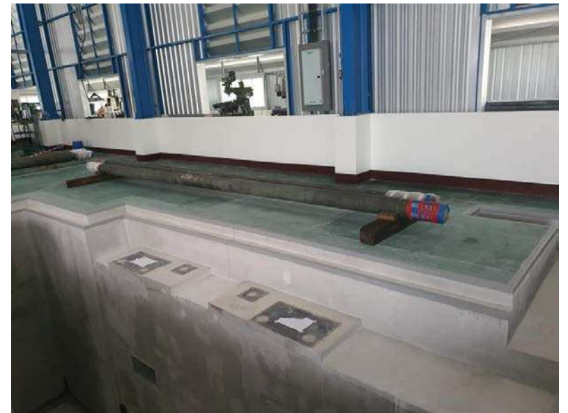
Foundation Pit for AIDA 1000 ton Press
